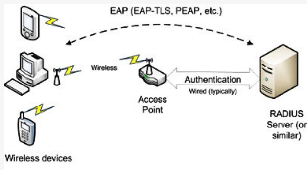
Figure 2. Enterprise WiFi Authentication
